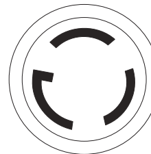
Figure 2-7. 120 VAC, 30 Amp Receptacle NEMA L5-30R
